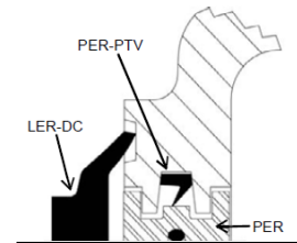
The LER-DC Dust Cover Can Be Used with LER and PER Seals. Available from Sizes 517-544, These Seals Act as a Flinger Against Contaminants
