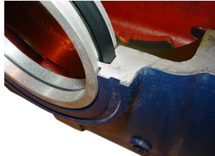
PER PTV-ring is a Contact Lip Seal Installed Over the PER for Added Protection
