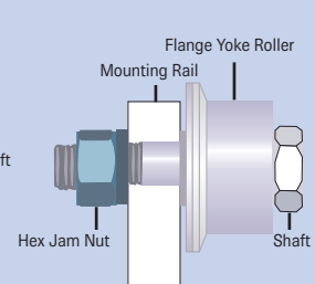
Through-Hole Mount Yoke Type
