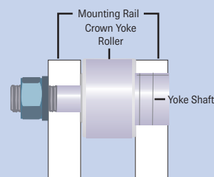
Captured Mount Yoke Type
