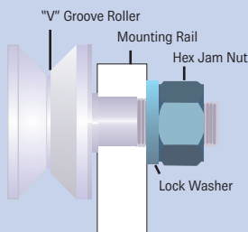
Through-Hole Mount Stud Type
